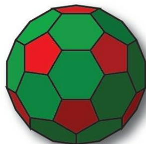
TRUNCATED ICOSAHDRON
