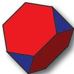
TRUNCATED TETRAHEDRON
