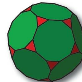
TRUNCATED DODECAHDRON
