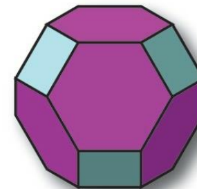
TRUNCATED OCTOHDRON
