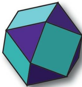
CUBOCTOHDRON
