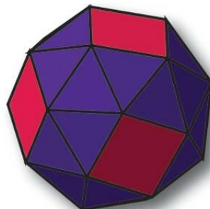
SNUB CUBE
