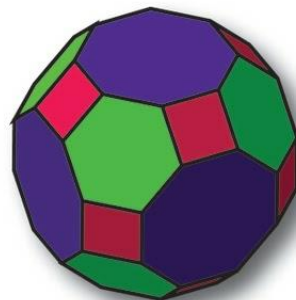
TRUNCATED CUBOCTOHDRON
