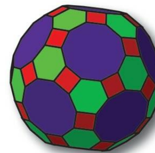
TRUNCATED ICOSIDODECAHDRON
