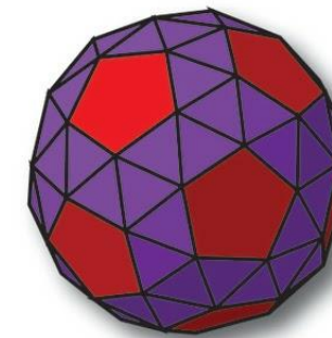
SNUB DODECAHDRON
