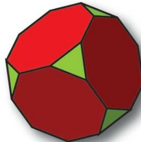
TRUNCATED CUBE
